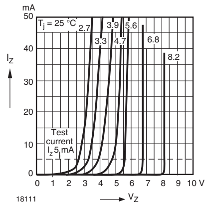
Fig. 14 - Breakdown Characteristics
