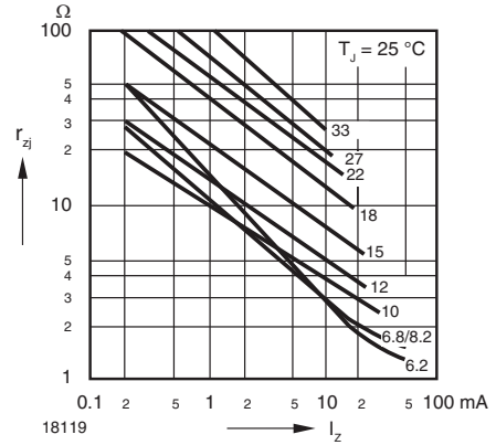
Fig. 4 - Dynamic Resistance vs. Zener Current
