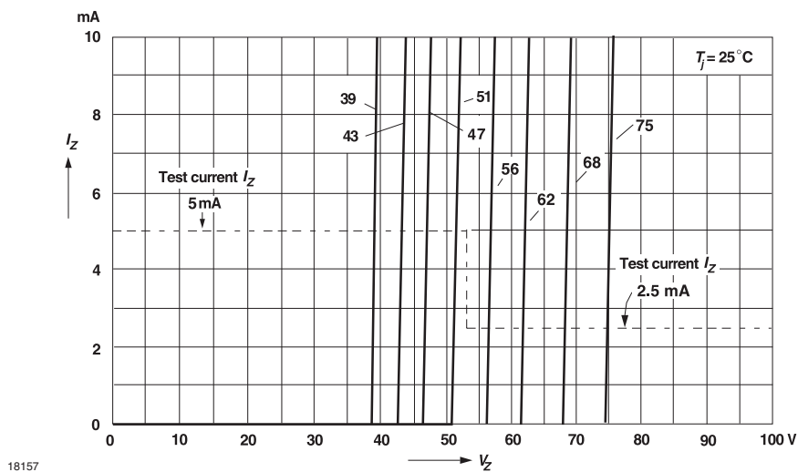
Fig. 16 - Breakdown Characteristics
