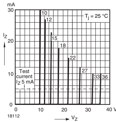
Fig. 15 - Breakdown Characteristics
