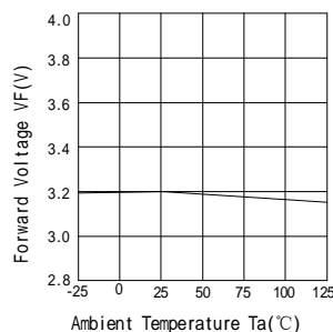
Forward Voltage vs. Ambient Temperature
