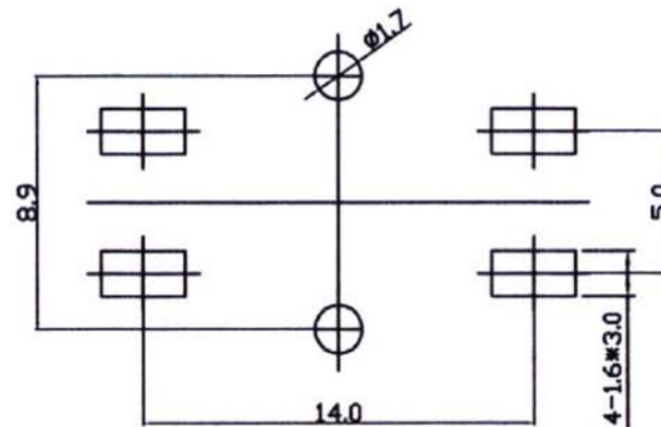
PCB DIMENSION
