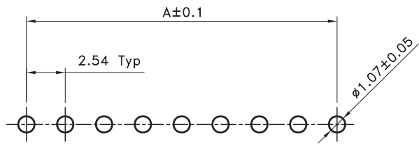
Recommnd PCB Layout
