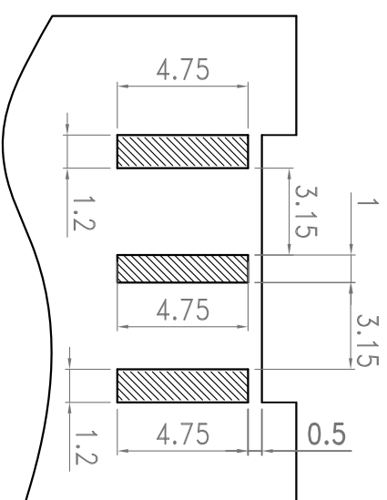
Recommended PCB Soldering Pattern
