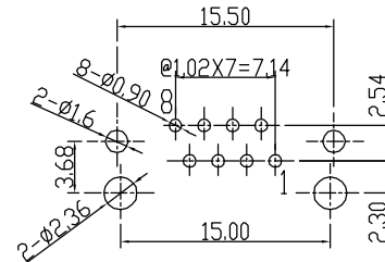
PC BOARD LAYOUT THICKNESS=1.6MM
