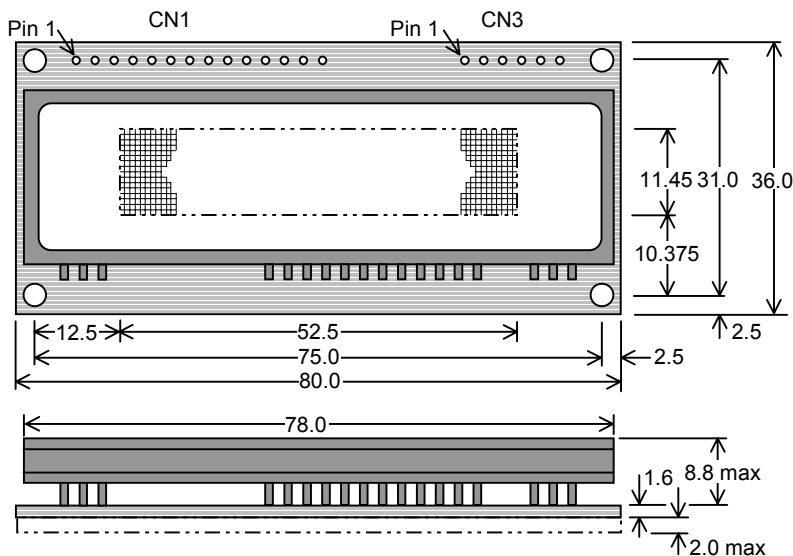
Dimensions in mm & subject to tolerances. Mounting holes 3.0mm dia.
