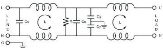
电气原理图(Electrical Schematic): 35
