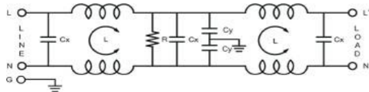
电气原理图(Electrical Schematic): 22
