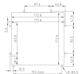
PANEL CUTOUT
