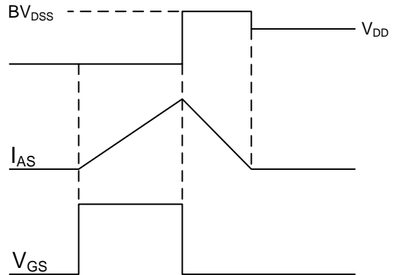
Fig.10 EAS Waveform
