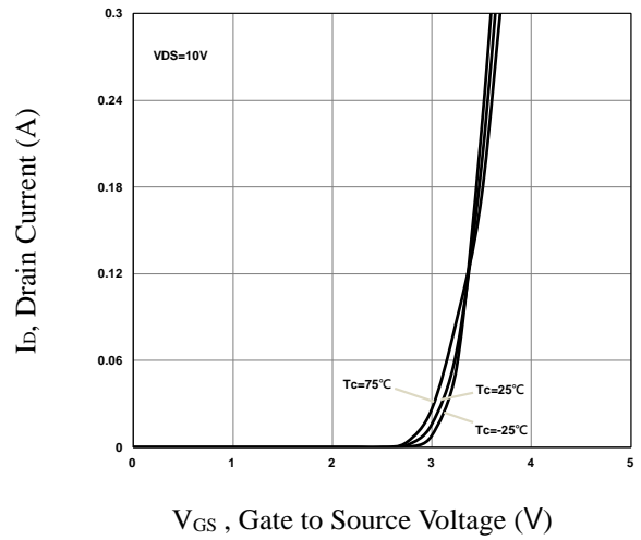
Fig.8 Transfer Characteristics
