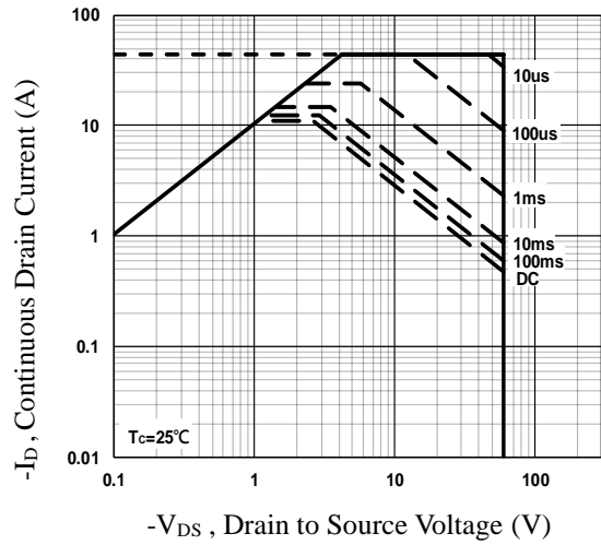
Fig.20 Maximum Safe Operation Area
