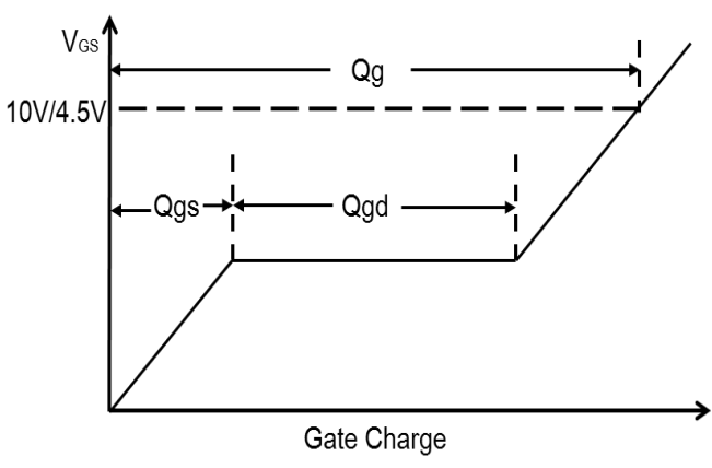
Fig.11 Gate Charge Waveform
