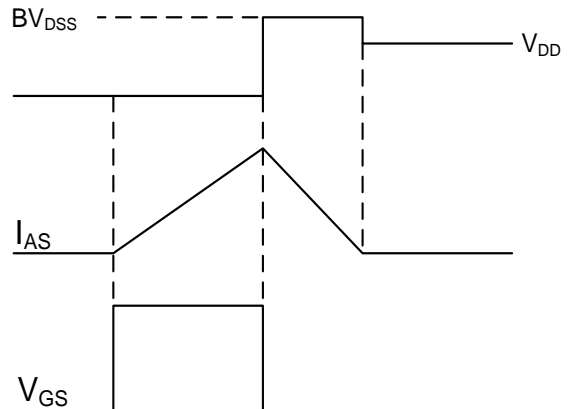
Fig.11 EAS Waveform
