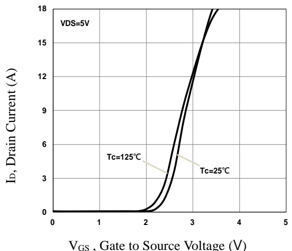
Fig.10 Transfer Characteristics
