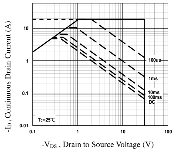
Fig.24 Maximum Safe Operation Area
