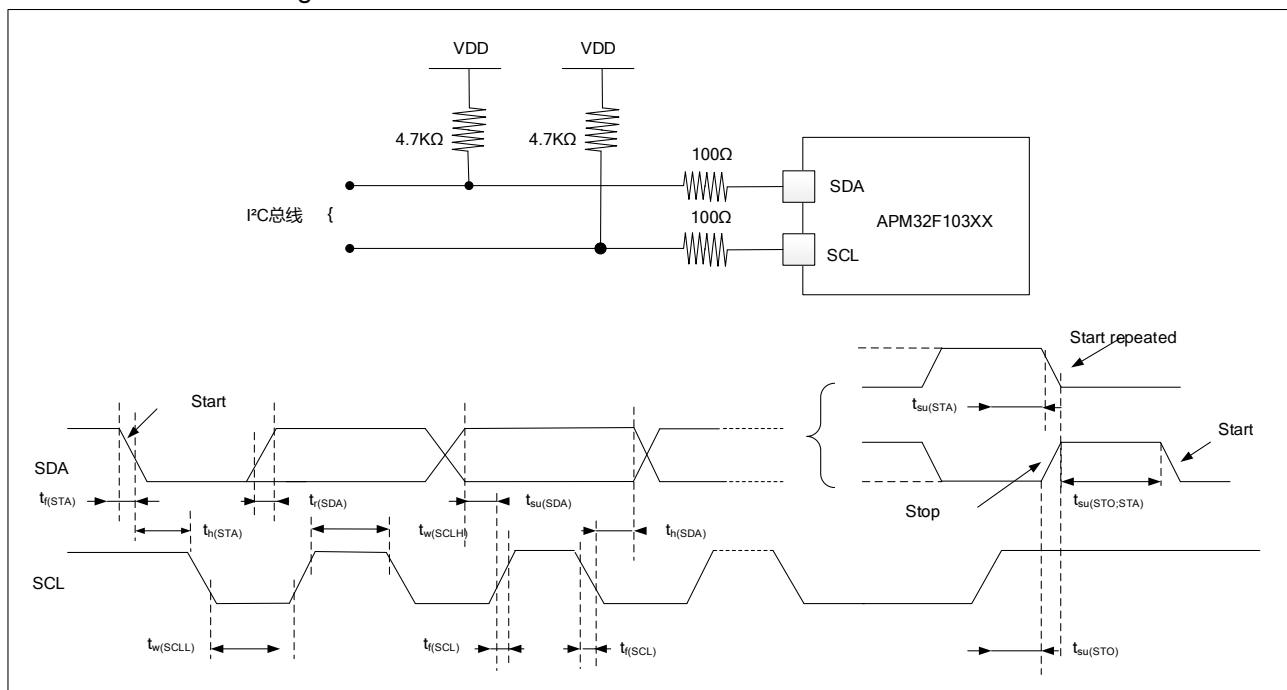
Figure 15. Bus AC Waveform and Measurement Circuit (1)
