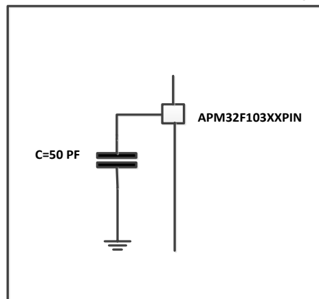
Figure 9. Load Conditions When Measuring Pin Parameters
