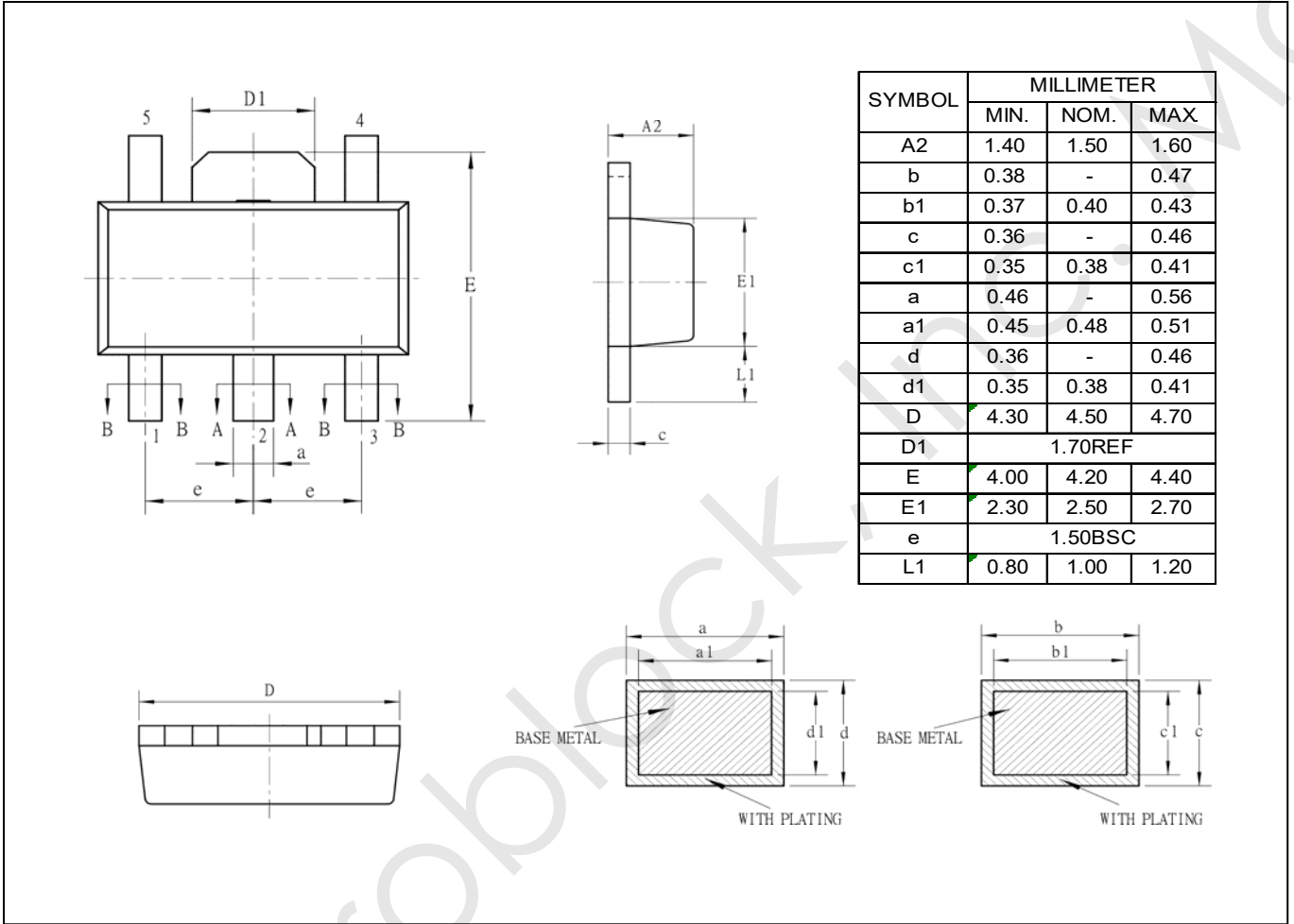
MBI6663GSB Outline Drawing
