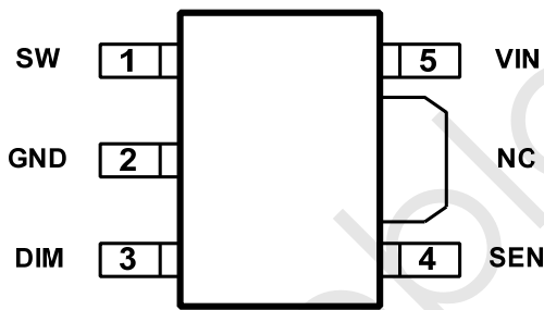
MBI6663GSB (Top View)
