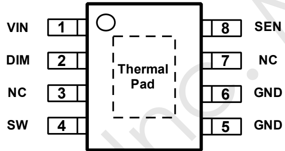
MBI6663GD (Top View)
