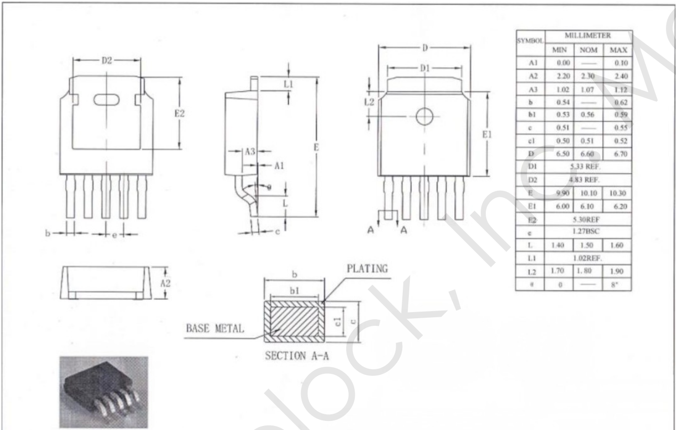
MBI6663GSD Outline Drawing
