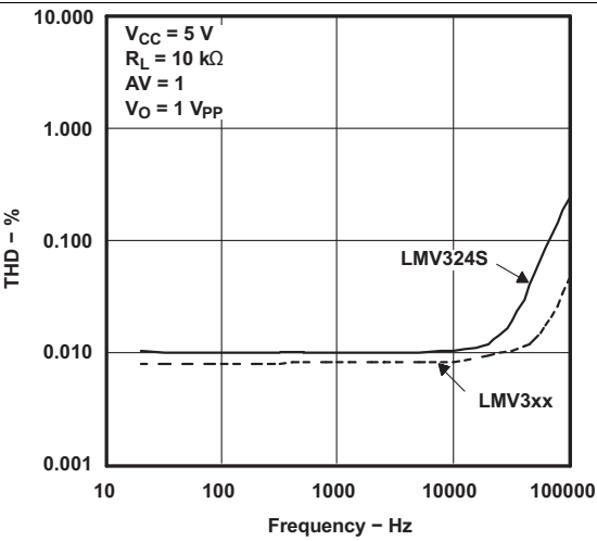
Figure 39. THD + N vs Frequency
