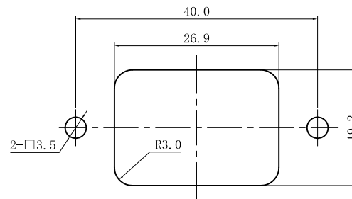
PANEL CUT-OUT
