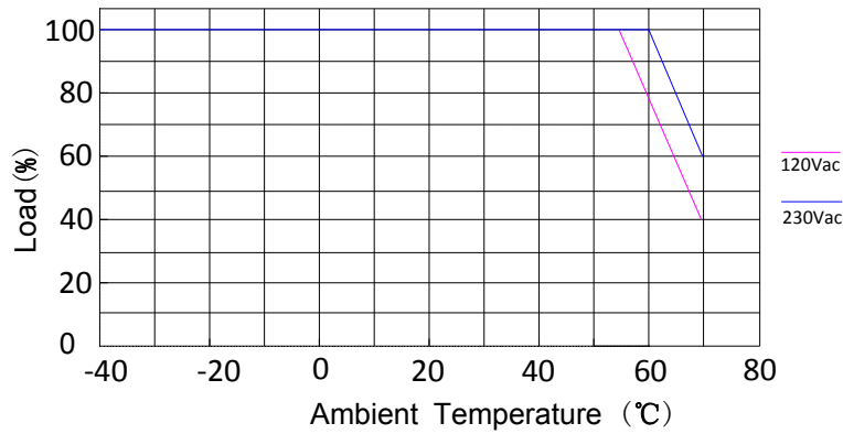
Derating Curve
