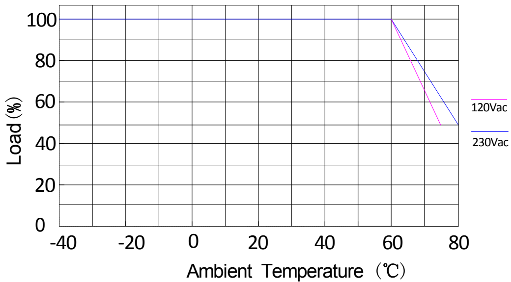
Derating Curve
