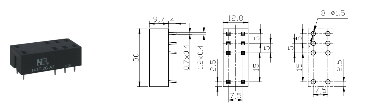
141FF-2C-A2 Dimension PCB layout
