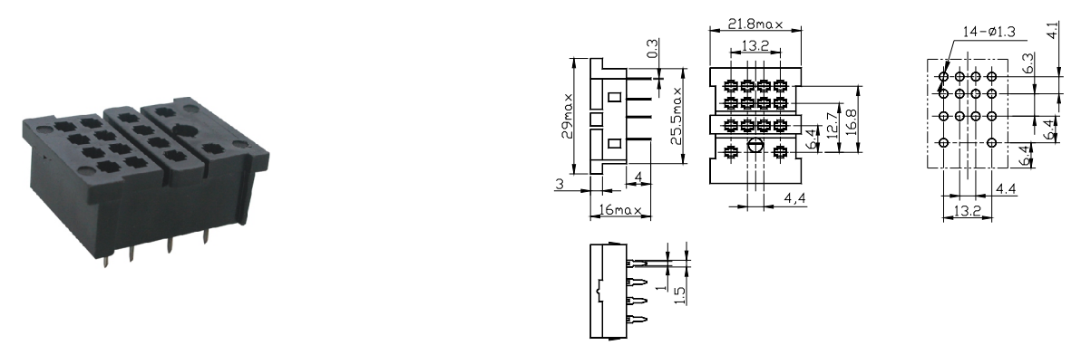
18FF-4C-D1 Dimension PCB layout Inter Connection
