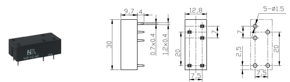
14F-1C-A2 Dimension PCB layout
