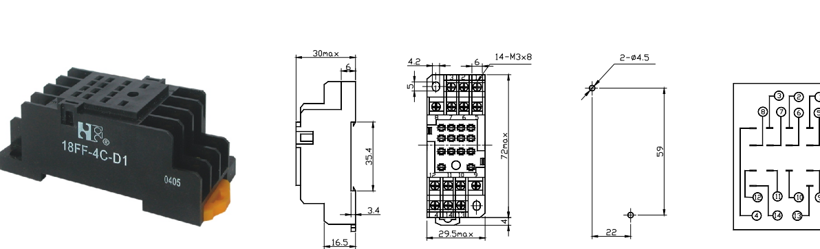
18FF-4C-D1 Dimension PCB layout Inter Connection
