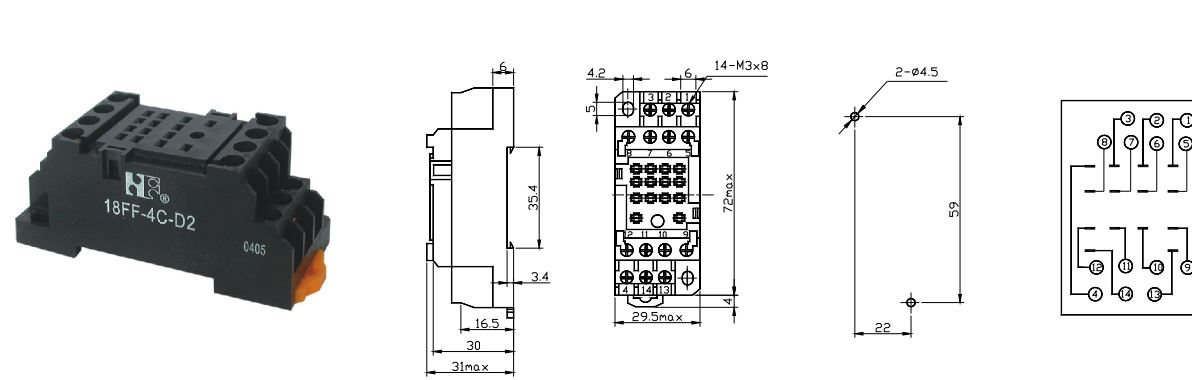
18FF-4C-D2 Dimension PCB layout Inter Connection
