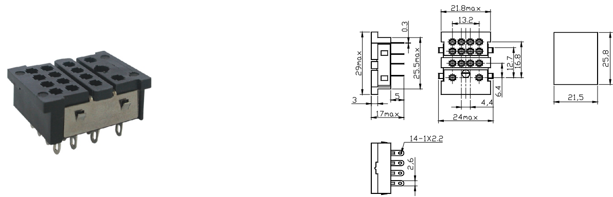
18FF-4C-A2 Dimension Mounting Holes
