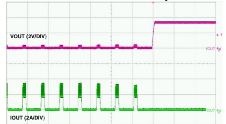
Time-5ms/div
