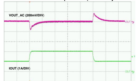
Time-100μs/div
