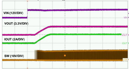
Time-500μs/div
