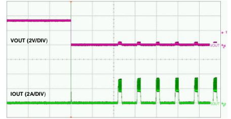
Time-5ms/div
