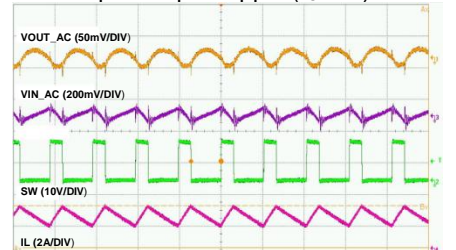
Time-2μs/div
