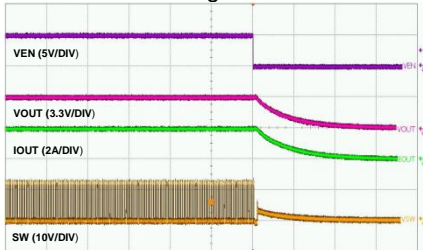
Time-50μs/div
