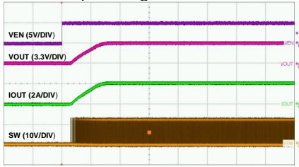
Time-500μs/div
