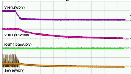
Time-500ms/div
