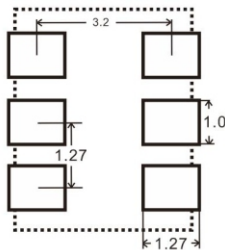
Figure 8. Recommended design size of AHT10 PCB (mm) and the outer part with dotted line is the outer dimension of SMD package.
