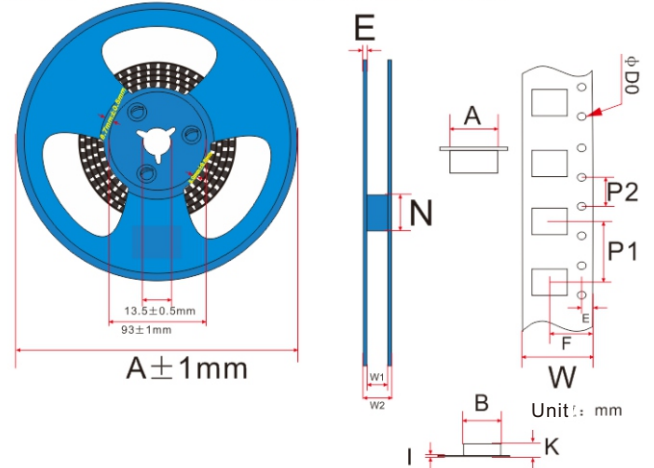
Figure 20 Package tape and sensor location diagram
