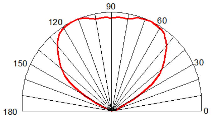
Fig.8 Radiation pattern@350mA
