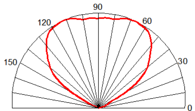
Fig.8 Radiation pattern@150mA
