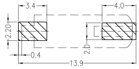
Board Layout
