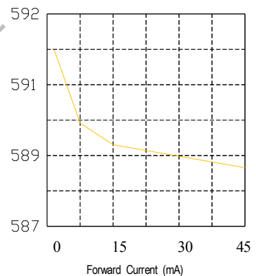
Forward Current vs. Dominate wavelength (Ta=25°C)
