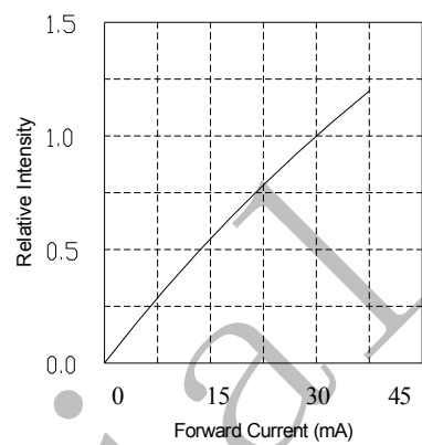
Relative Intensity vs. Forward Current (Ta=25°C)
